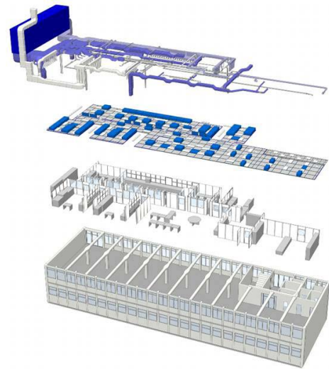
Example of a cleanroom system by ASYS Cleanroom
